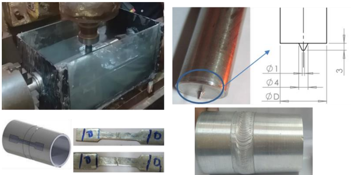
Figure 1. EG-FSW-M1 equipment, UWFSW of AA 6061 pipes.
